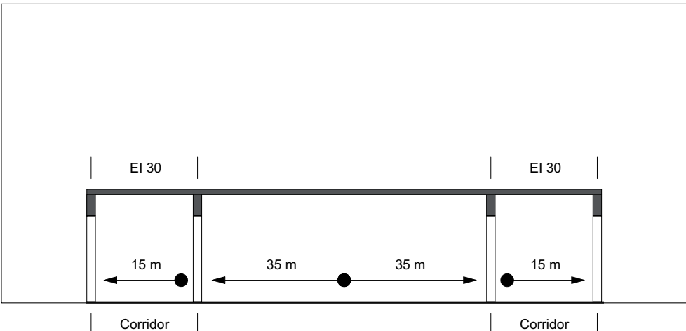
Escape route length with several exits with additionally protected corridors (EI 30) 35 m + 15 m = 50 m
